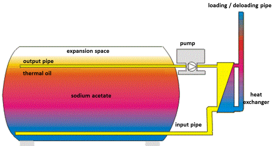
Figure 21: Scheme of a latent heat storage system (adapted from TransHeat GmbH)
