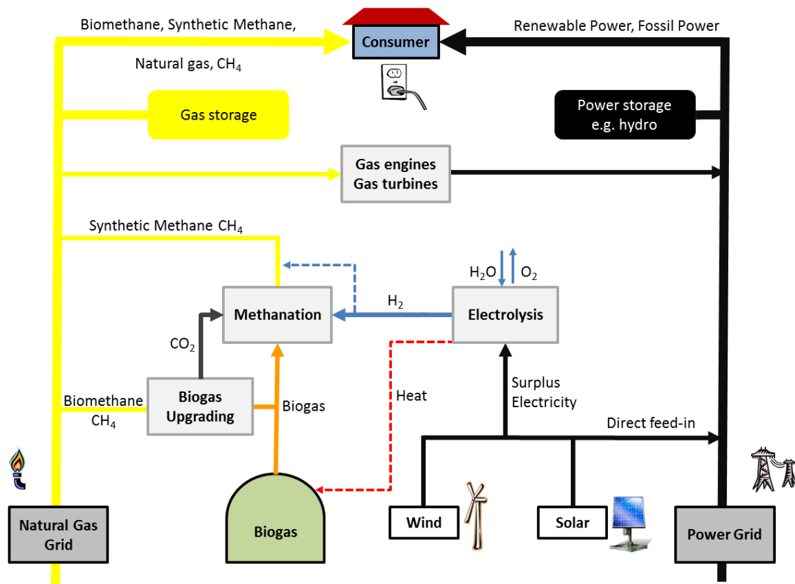
Figure 47: Power-to-Gas concept
